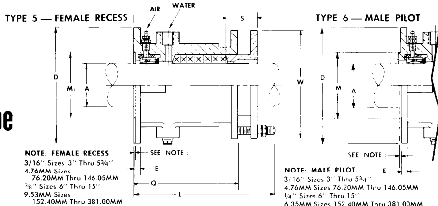
NOTE: FOR FLANGE HOLES SEE DRILLING DIAGRAM ON PAGES 746 AND 747 (FIG. 1788IR AIR-WATER SERVICE)
