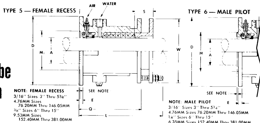
(FIG. 1788 IR AIR-WATER SERVICE)
