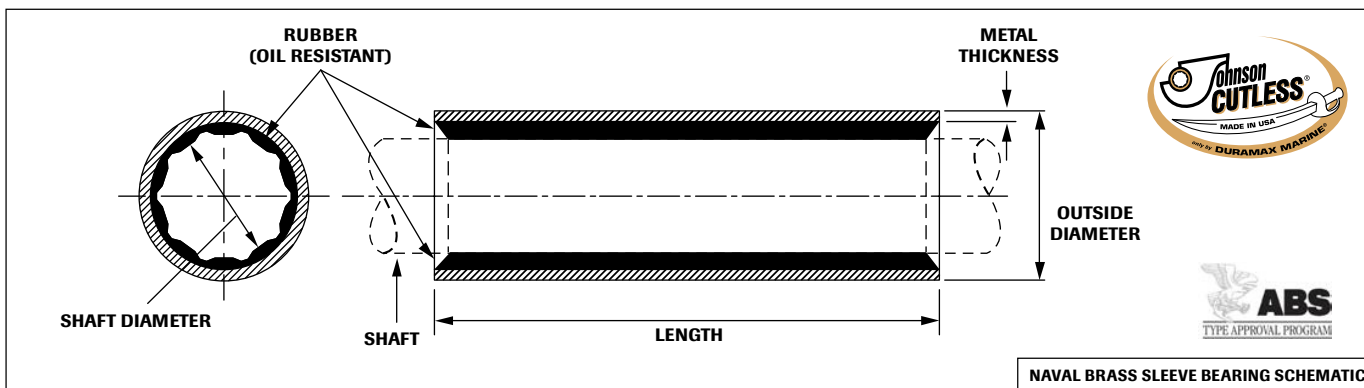
NAVAL BRASS SLEEVE BEARING SCHEMATIC
