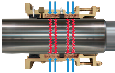
Flax packing acts as insulator trapping heat to shaft.
