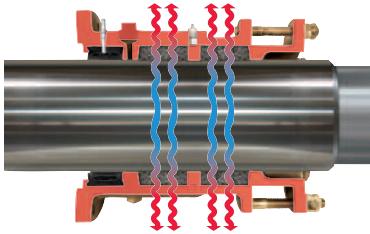
Duramax® Ultra-X Packing transfers heat to stuffing box.
