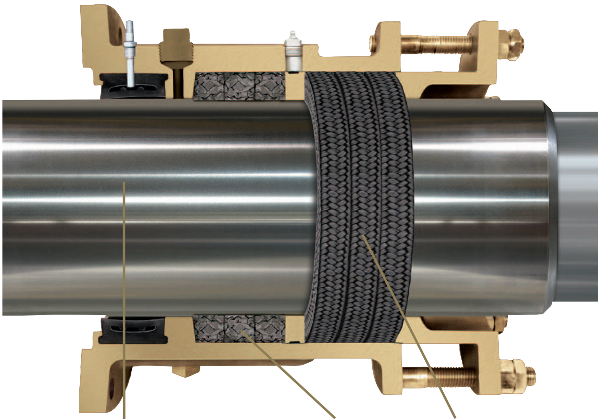
Duramax® Ultra-X Packing transfers heat to stuffing box.
